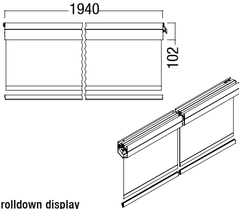
RW9000 Fabric roll-down display Includes M816 roll-down wall, base plates, uprights and horizontals Case not included
