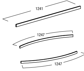
Beam (M 1354.01/USA) OP 181.01/USA beam straight OP 183.01/USA beam curved concave OP 185.01/USA beam curved convex
