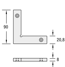
Z 966/S Internal corner connector for OCTAfabric
