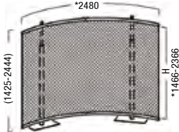
OP 904 Banner set curved concave 2 telescopic uprights and 4 beam extrusions 1240 mm long, incl. 2 base plates
