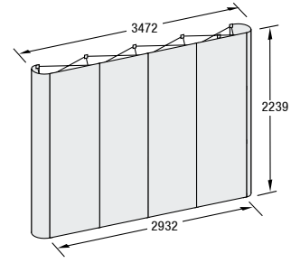
VA 4743 P1 straight, for 4 panels
