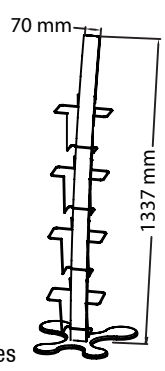
P-L4 Literature rack with 4 pouches without transport bag
