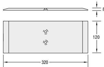
M 1398 Base plate steel for M-Set 1307 incl. screw set M8 x 60
