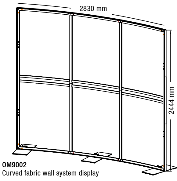
Frame Dimensions
